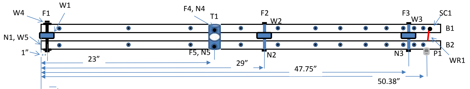
Side View
